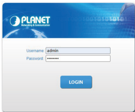
Figure 5-6: Login Screen
