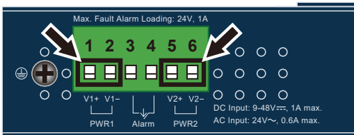
Figure 3-4: IGS-4215-4T2S Inlet Power Socket
