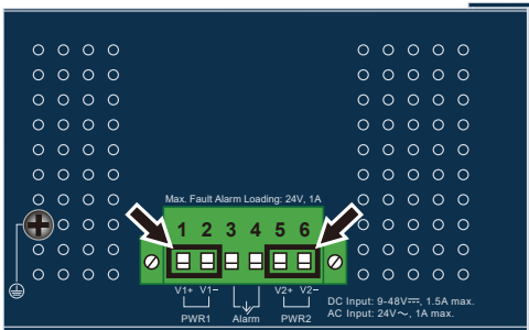
Figure 3-2: IGS-4215-16T2S-U Inlet Power Socket
