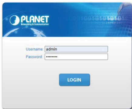
Figure 5-4: Login Screen
